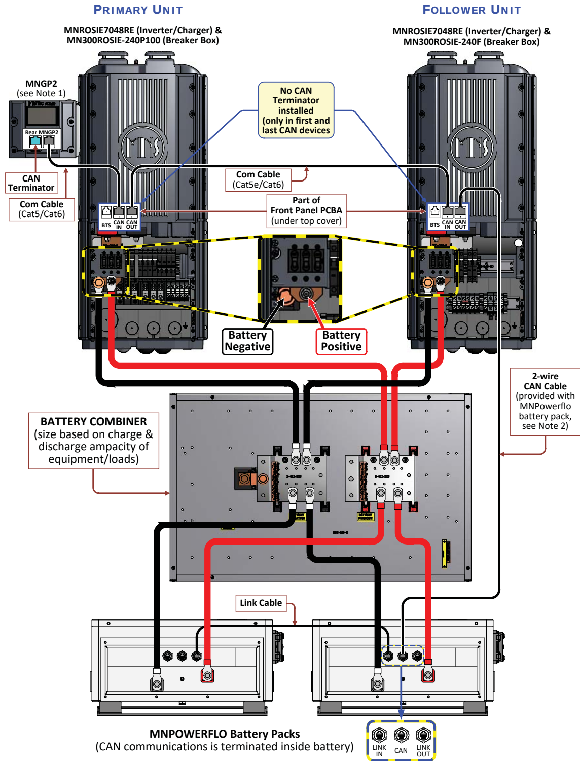
Figure 6, DC Wiring with Closed-Loop Communications - Parallel Stacked Rosie Inverters
