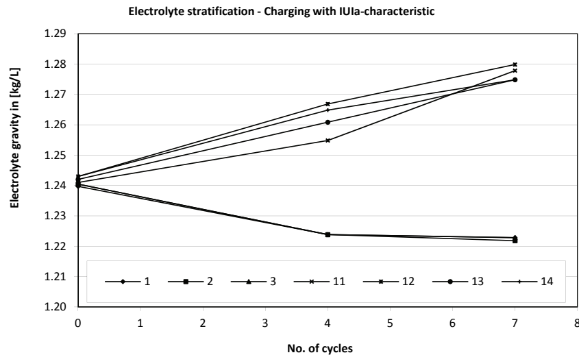
Figure 7a - Recharge with IU1a-characteristic without mechanical electrolyte mixing
