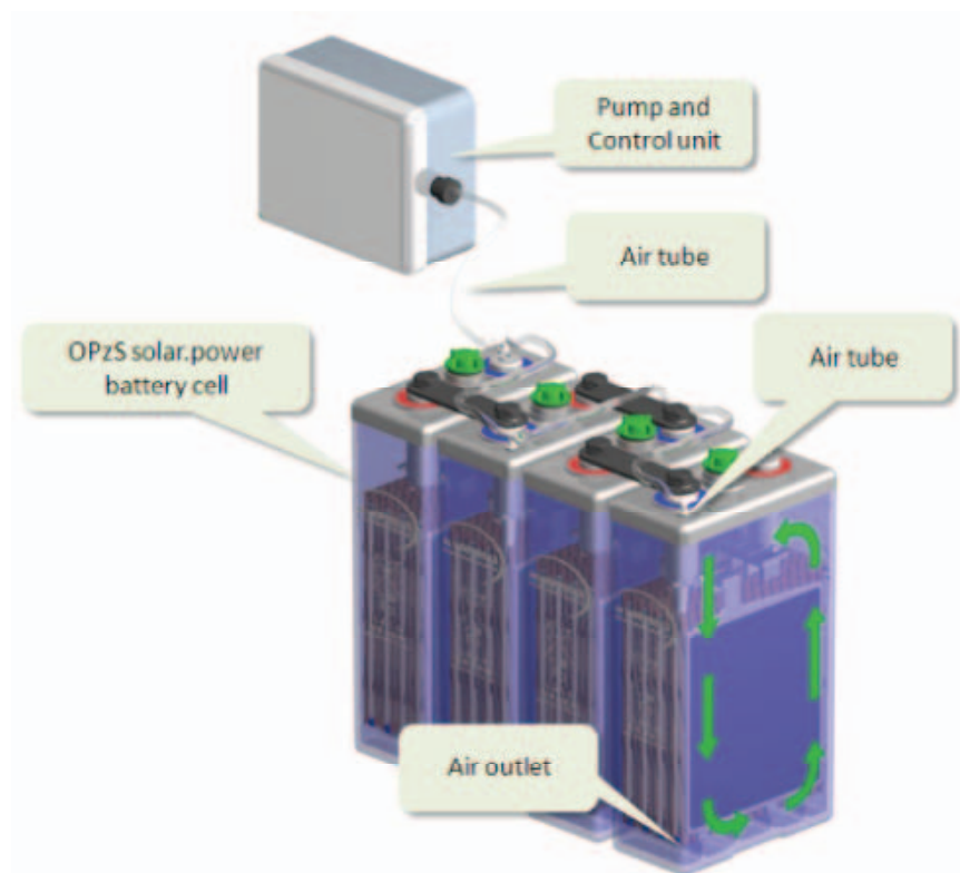
Figure 5 - Electrolyte recirculation system (system overview)
