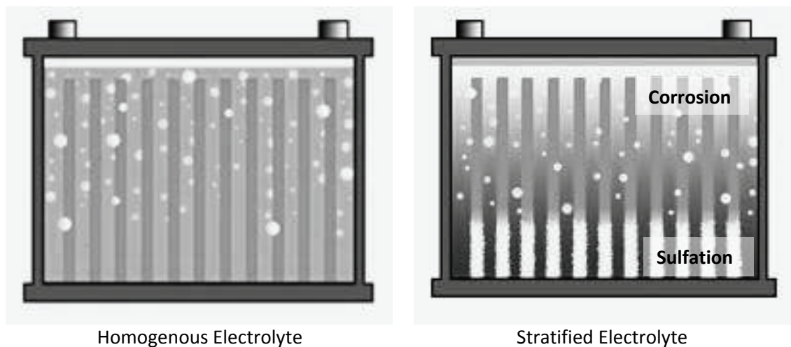
Figure 2 - Consequences of electrolyte stratification on lead acid batteries
