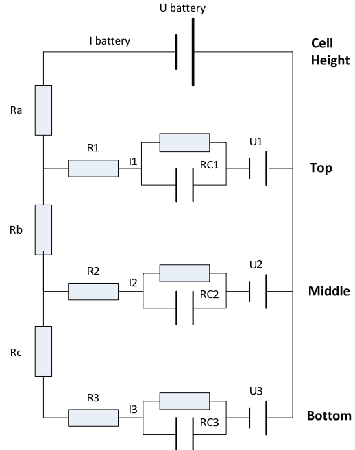
Figure 1 - Equivalent circuit diagram of an electrode
