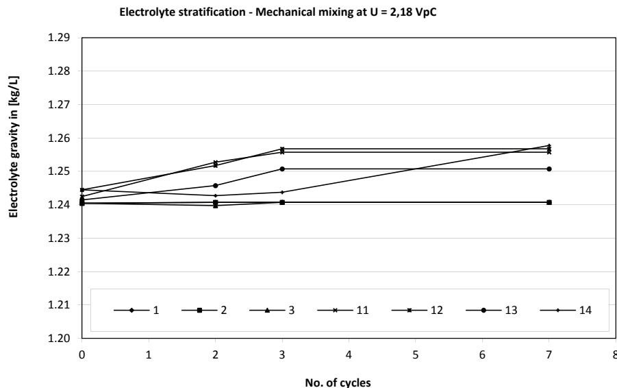
Figure 7b - Recharge with IU-characteristic with mechanical mixing of the electrolyte starting at U = 2.18 V/Cell.
