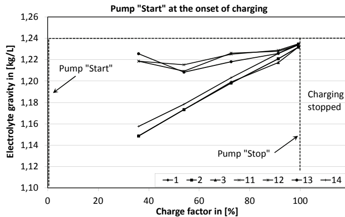
Figure 6a - continuous pump operation during charging
