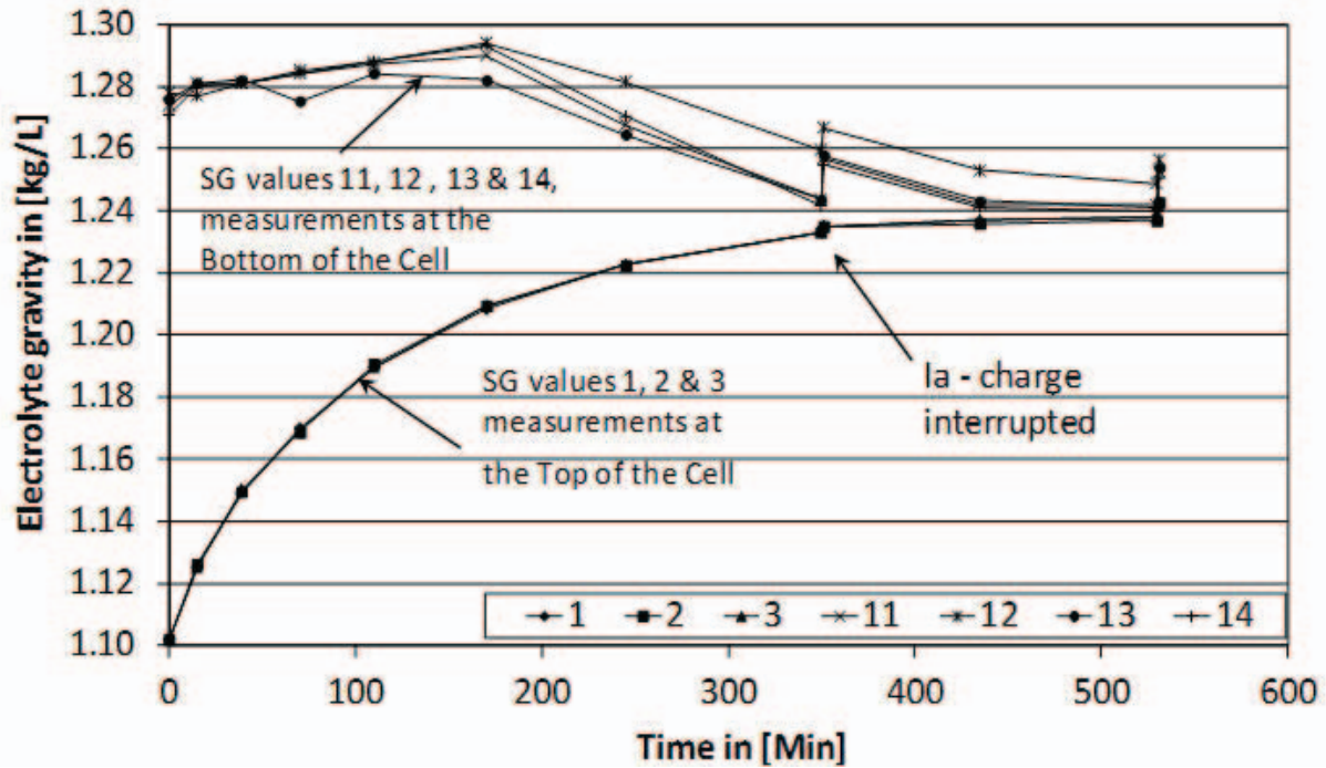
Figure 4 - Electrolyte mixing using an Ia-charging with 5A/100Ah (150A) after 5 cycles with IU charging
