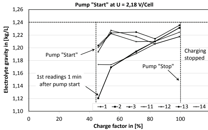
Figure 6b - pump starting only after charge voltage reaches 2.18 V/cell
