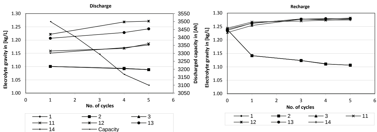
Figure 3 - Electrolyte stratification of a 3219Ah tubular positive plate battery after cycling
